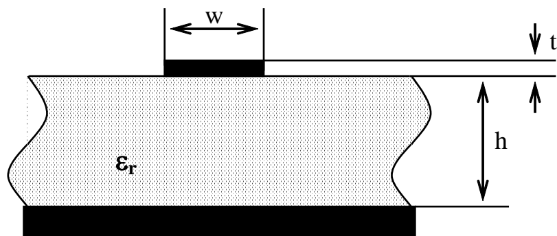
Linia microstrip
